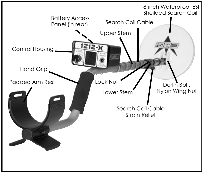
Figure 1. Fisher M-Scope 1212-X
