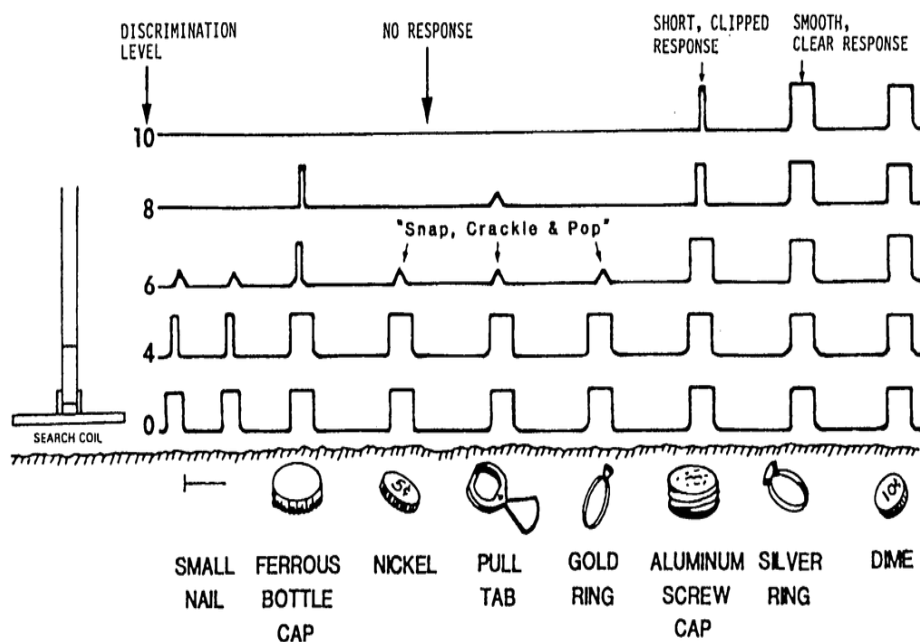
Figure 4. Typical 1212-X audio responses over 1-inch deep targets with search coil sweeping 2 to 3 inches above ground.
