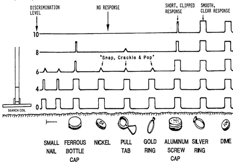
Figure 4. Discrimination. Typical 1225-X audio responses for 2-inch deep targets with search coil sweeping 1 to 2 inches above ground.
